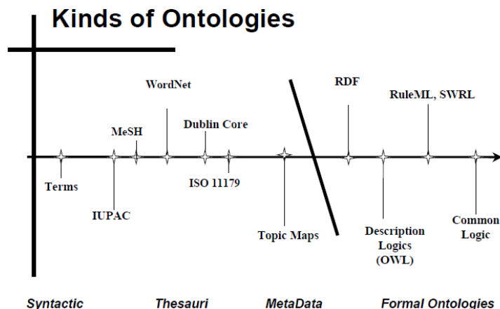
Figure 3: The Ontology Spectrum, originally developed by (Gruninger, et al., 1999).
