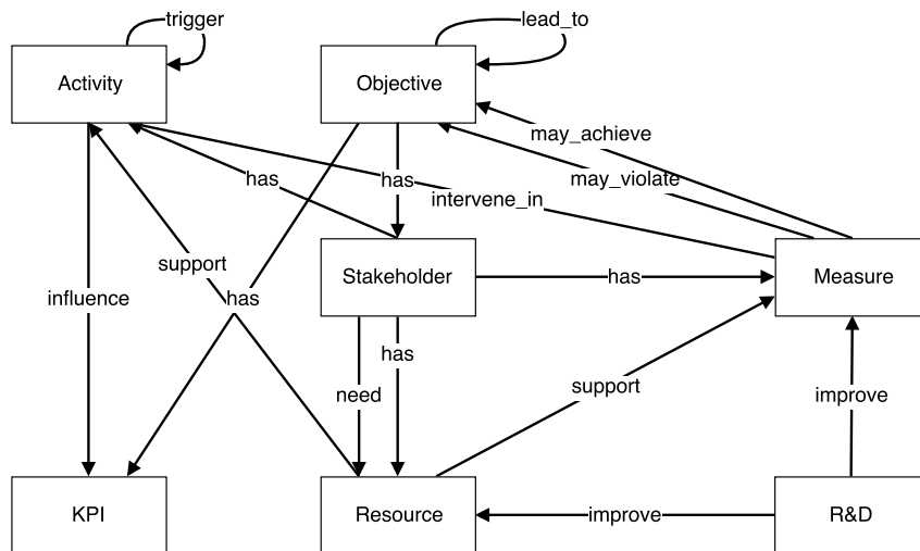
Figure 11: Top-level classes of GenCLOn, redrawn from (Anand, et al., 2012).
