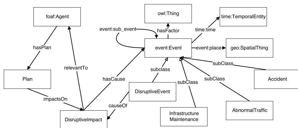
Figure 7: Depiction of the Transport Disruption Ontology, redrawn from (Corsar, et al., 2015). Reused classes are indicated with prefixes.
