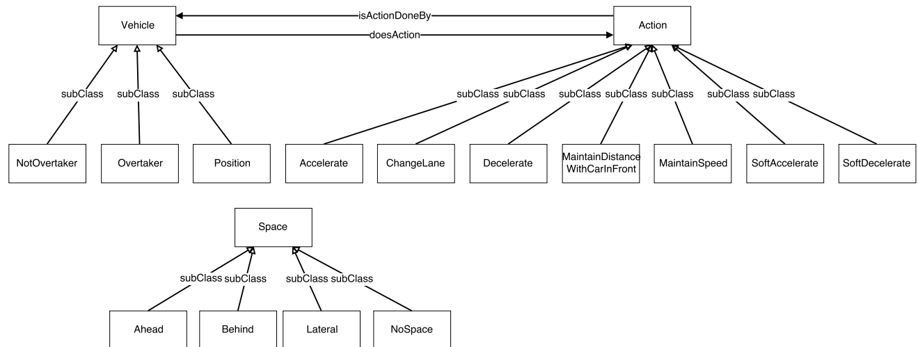
Figure 8: Depiction of the ontology for road traffic management.
