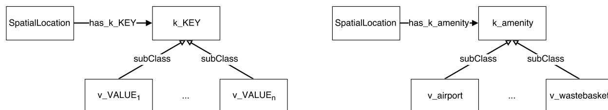
Figure 10: The generic structure (left) and an example (right) of the Osmonto representation of OSM keys.
