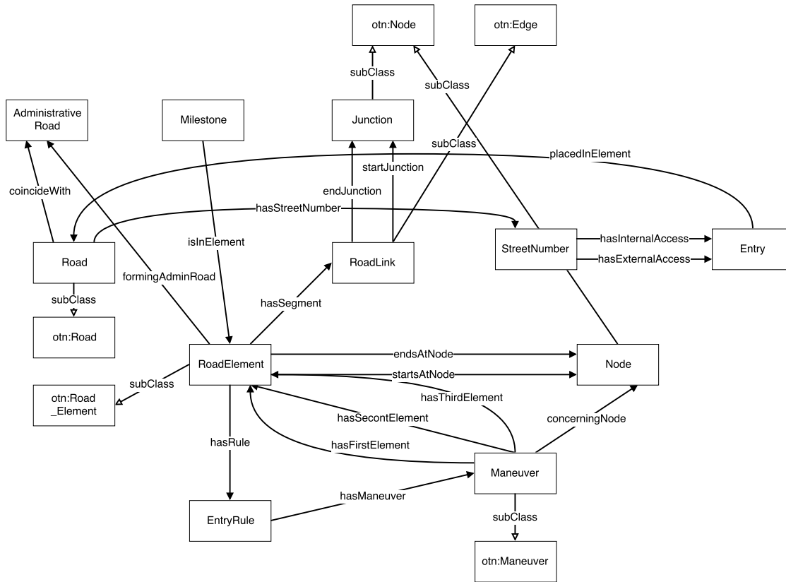
Figure 15: Depiction of the street-guide macroclass, reproduced from (Bellini, et al., 2014).
