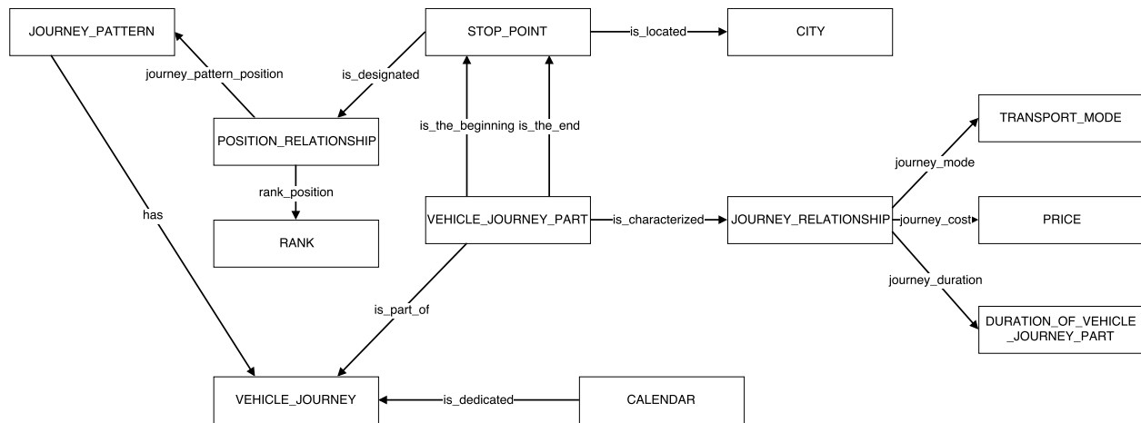
Figure 5: High-level concepts and relationships to characterize a journey.
