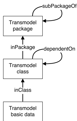
Figure 13: Depiction of the Transmodel ontology, redrawn from (Benvenuti, et al., 2017).
