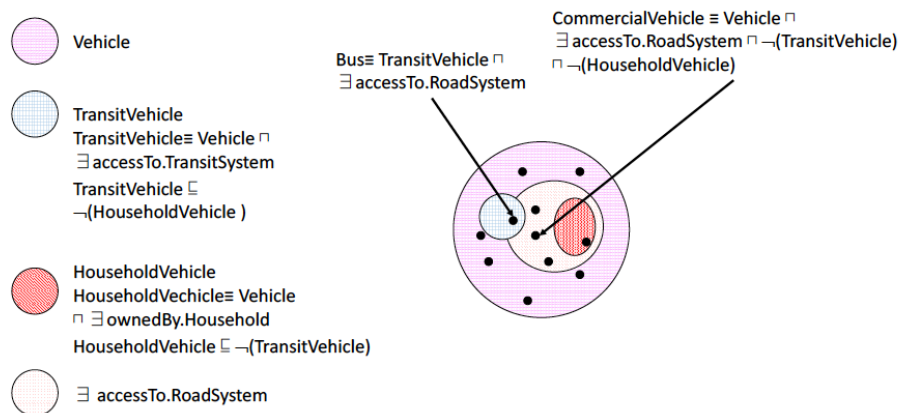
Figure 2: Example of an OWL representation of Vehicles.
