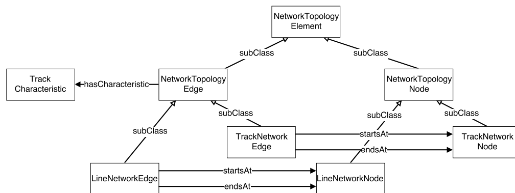
Figure 16: A high-level view of the Network Statement Checker ontology, reproduced from (Verstichel, et al., 2011).
