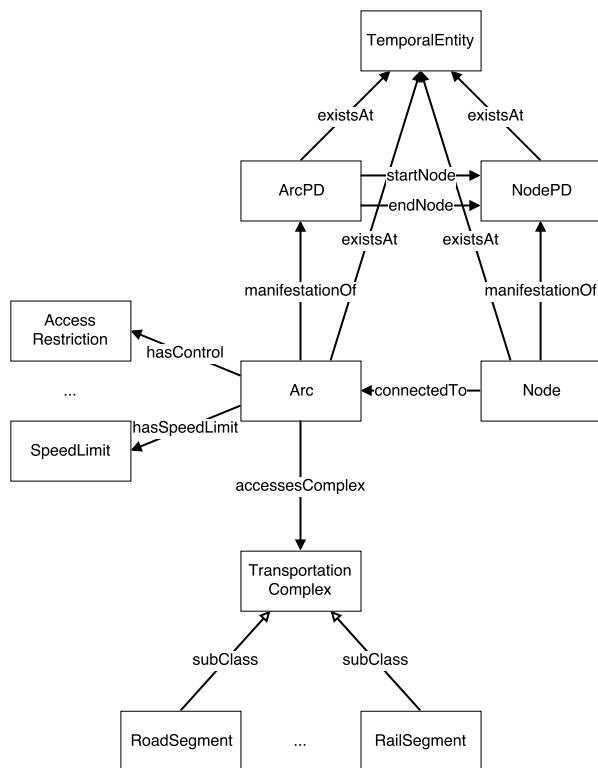
Figure 12: Structure of the iCity transportation network, redrawn from (Katsumi & Fox, 2017).
