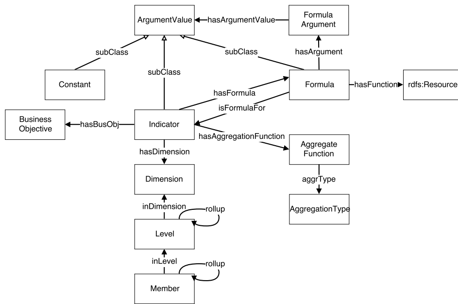
Figure 14: Depiction of the KPIOnto ontology, redrawn from (Benvenuti, et al., 2017).
