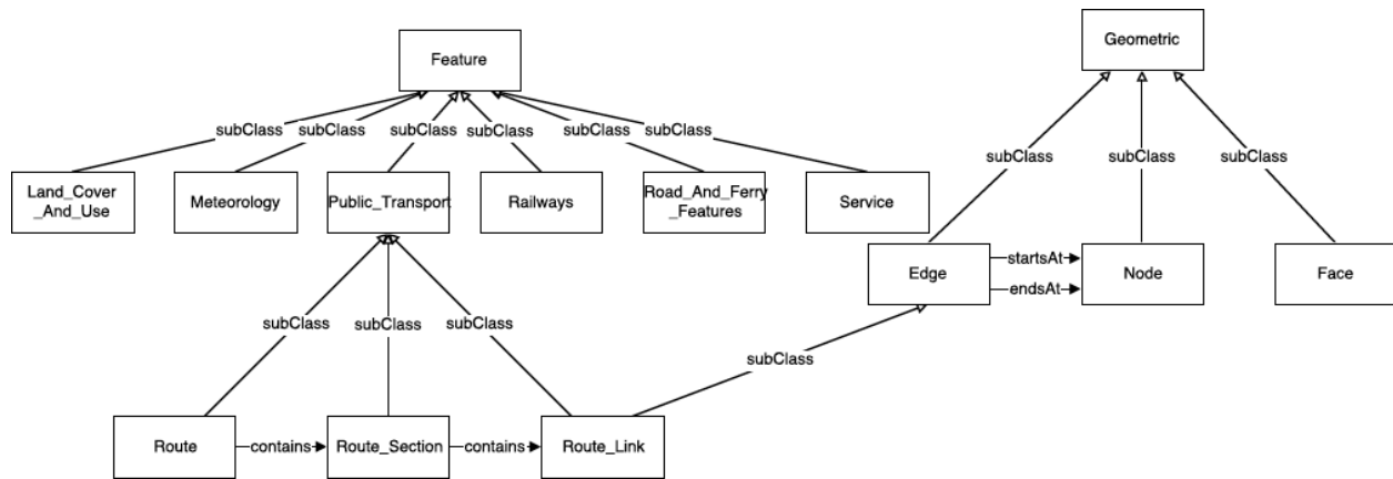
Figure 6: A selection of some of the basic classes in OTN, and their relationships.
