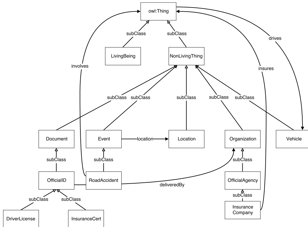
Figure 9: Depiction of the core classes and properties in the Road Accident Ontology.
