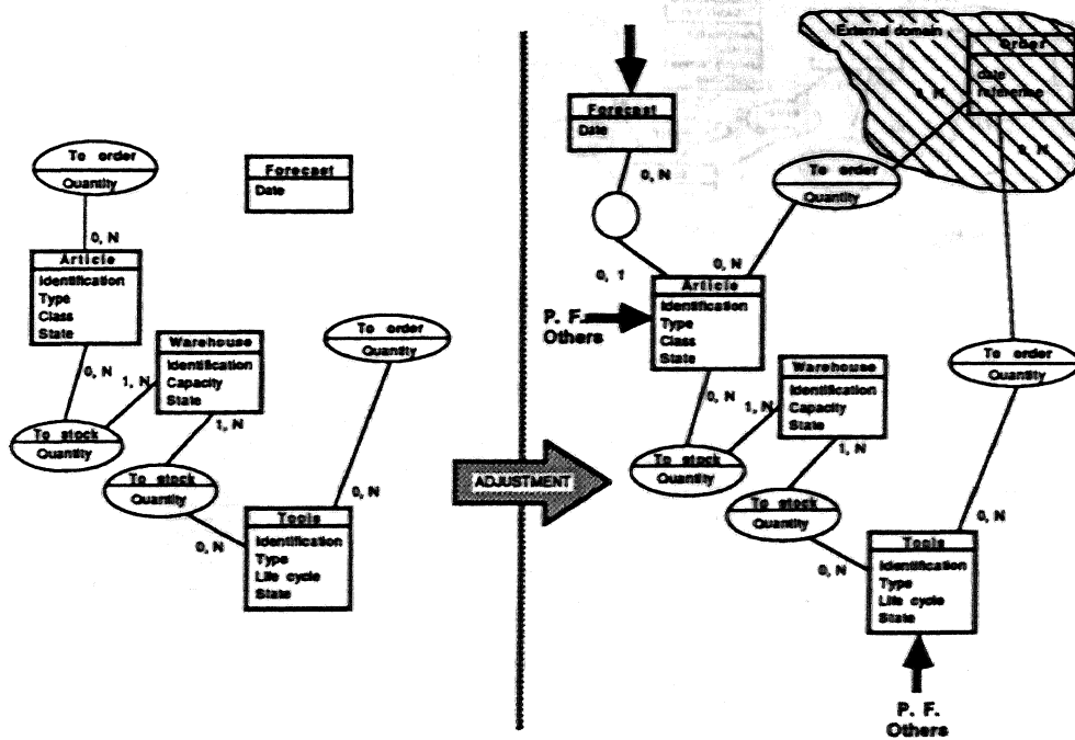
Figure 3-26: The supplying function conceptual data model
